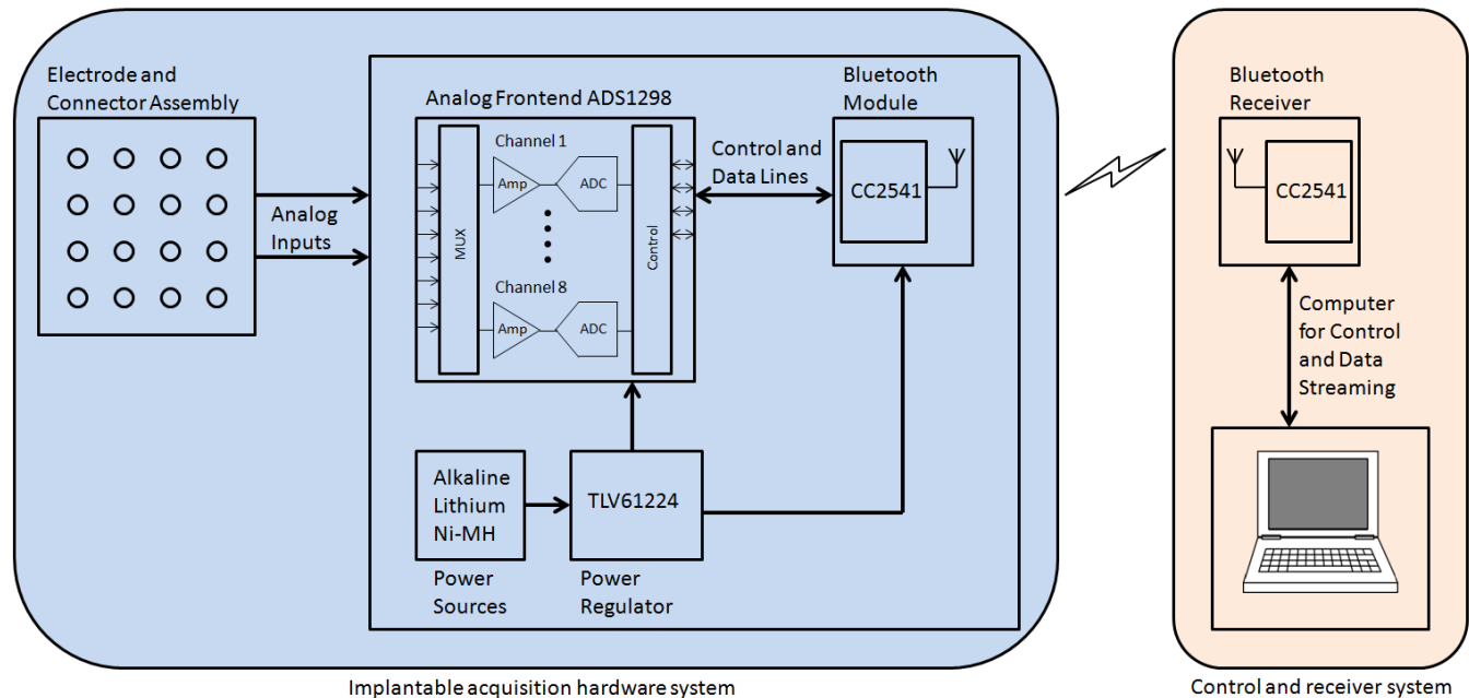
Figure 2: 8-channel wireless data acquisition system overall block diagram. The left block is the implantable wireless hardware. It contains the electrode and connector assembly along with the detachable wireless board. The analog signals are amplified and digitized with the analog frontend IC, ADS1298. The digital signal is then transferred to the Bluetooth module, CC2541, and packaged for wireless data transfer. The right block is the control and receiving system. It includes a Bluetooth receiver module and computer software system for acquiring the streamed data. Note that a custom Bluetooth receiver is not required for the receiving system. Devices such as laptops, smart-phones and tablets with built in Bluetooth 4.0 radio can be used.
